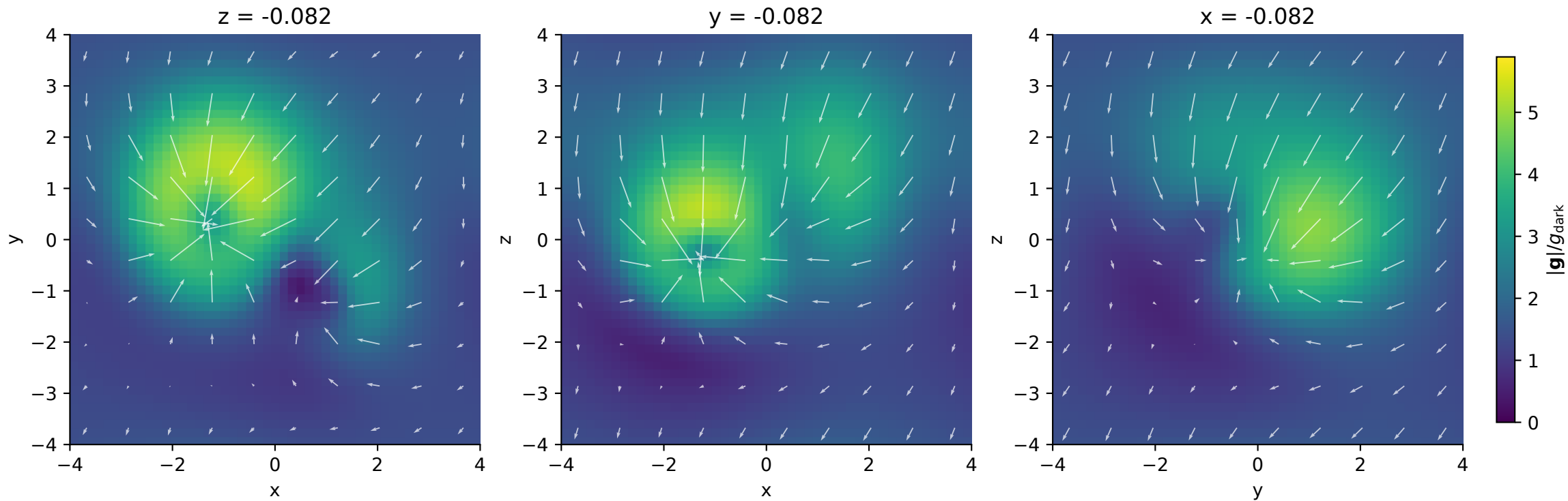
Three Cartesian slices of one nonsymmetric 49^3 solution Synthetic periodic density contrast; arrows show physical acceleration
