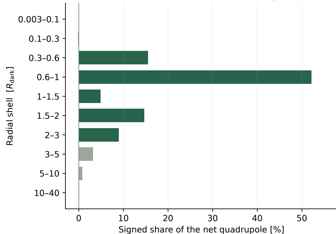
Where the local Poisson-source integral lies
