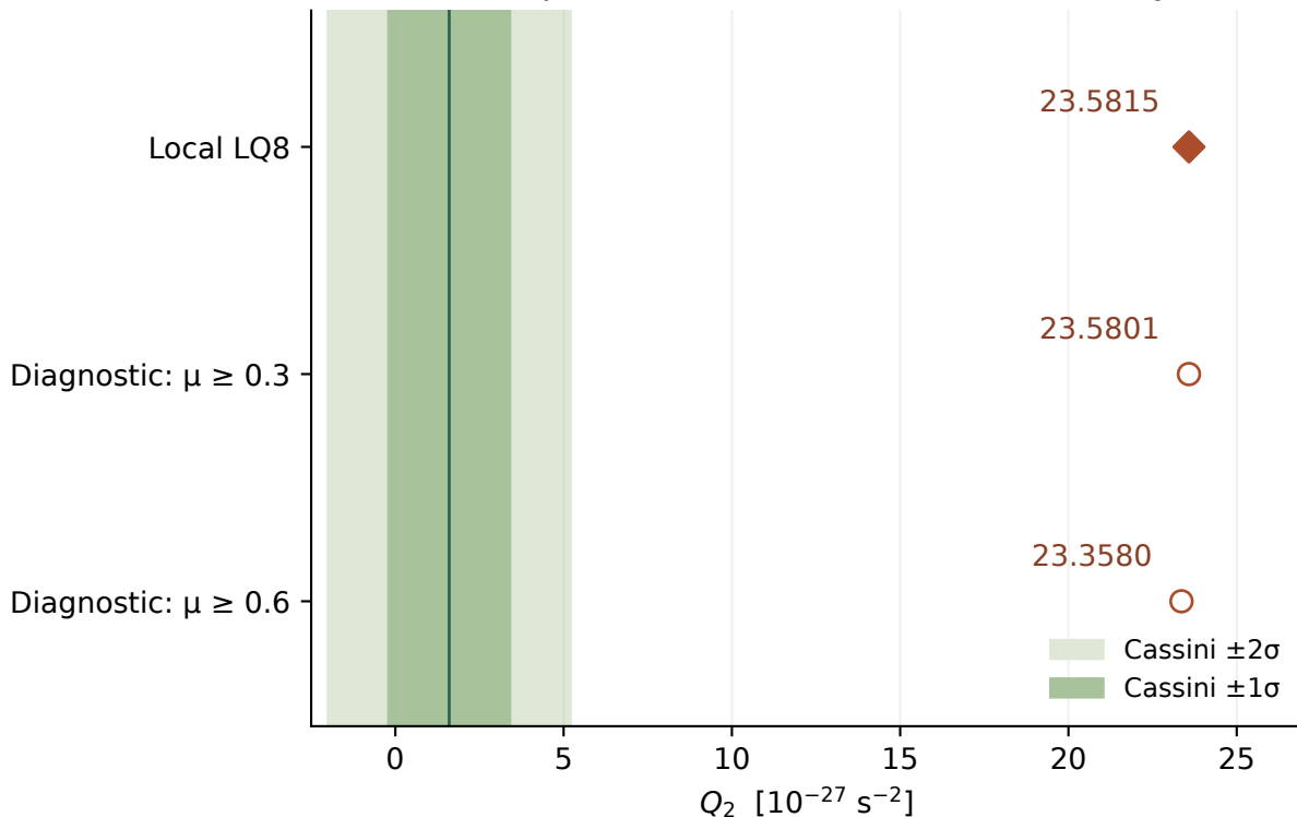
Solar prediction and weak-field sensitivity
